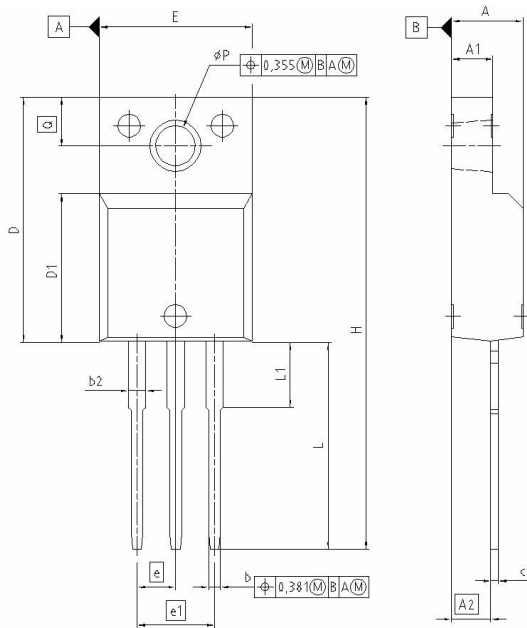
PG-TO220-3-31
